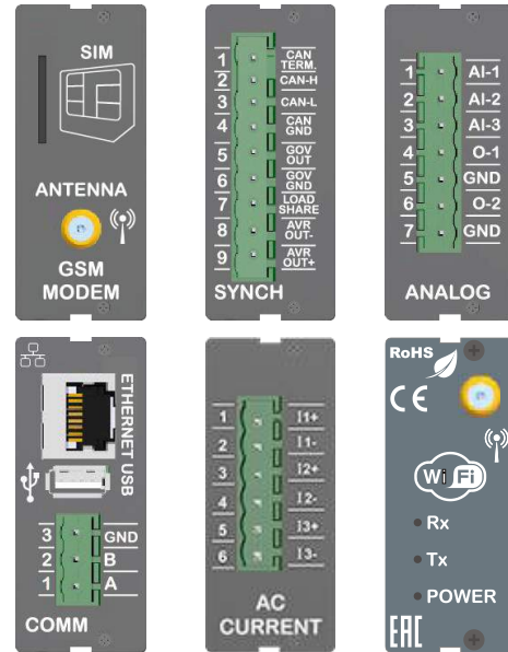
Plug-in modules
